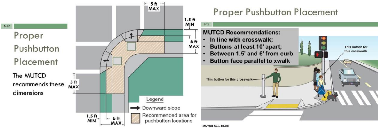
MUTCD Figure 4E-3
