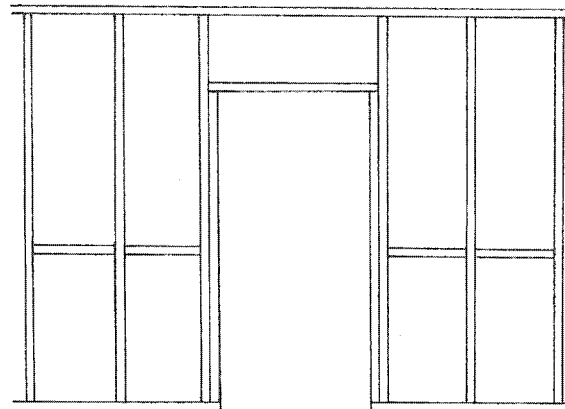
B. ADDING 2x4 BLOCKING BETWEEN STUDS AT THE LOCK LEVEL REINFORCES DOORFRAME.
