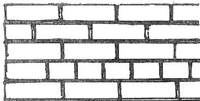
COMMON BOND
