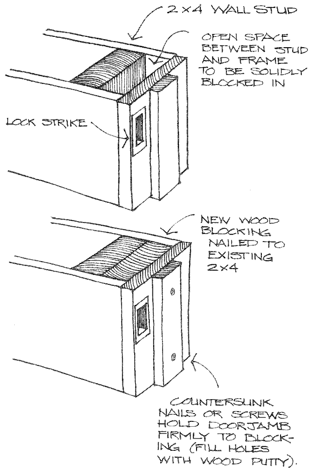
B. ADDING 2x4 BLOCKING BETWEEN STUDS AT THE LOCK LEVEL REINFORCES DOORFRAME.
