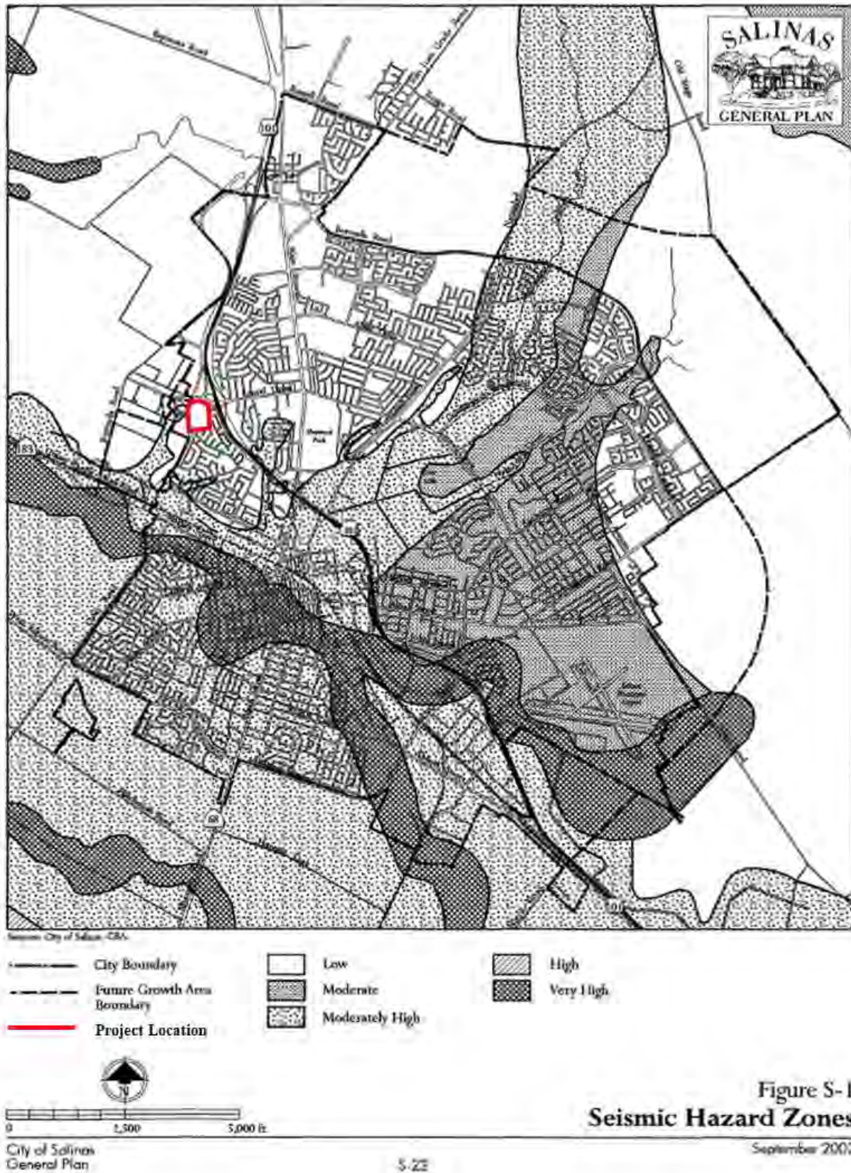
Figure 4-7 City of Salinas, General Plan, Seismic Hazard Zones
