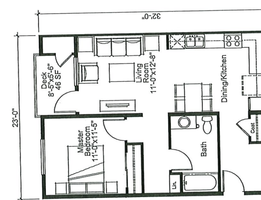
UNIT TYPE P1-1 1 BEDROOM / 1 BATHROOM #641 NET SF #743 GROSS SF
