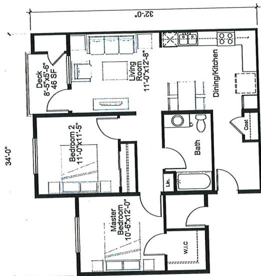
UNIT TYPE P2-1 2 BEDROOM / 1 BATHROOM ±838 NET SF ±950 GROSS SF
