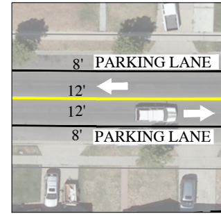
DETAIL B - TYPICAL STRIPING ALONG IRIS DR
