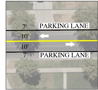
DETAIL C - TYPICAL STRIPING ALONG TYLER ST & HARDING ST
